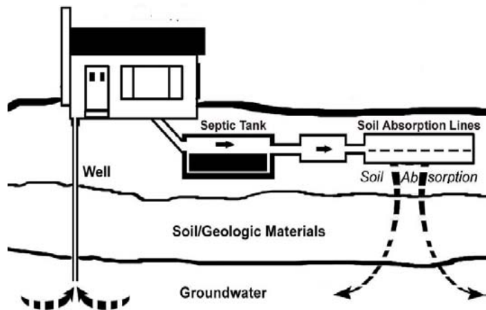
Conventional Septic Tank Drainfield System
