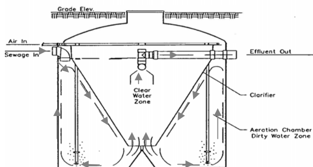
Aerobic Treatment Unit: Delta Environmental Products
